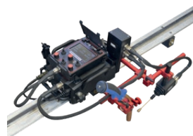
RAIL TITAN • Suitable for TIG welding (HF resistant) • Remote control pendant • Linear torch oscillator • Automatic seam tracking system
