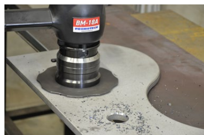
Bevel on holes from 40 mm in diameter
