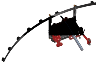
Following guide arms 20 x 20 mm for 36 mm wide flexible track (set of 2 pcs) PRW-0476-50-01-00-1
