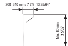
Large clamp for bulb profiles 200 - 340 mm (option) DCS-0824-0037-03-0
