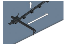
Guide adjustment tool to position 36 mm wide flexible track parallel to the edge UST-0466-53-00-00-0
