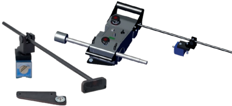
Circle Cutting Attachment for 240-1000 mm (9 29/64"-39 3/8") radius CYR-0475-22-00-00-0
