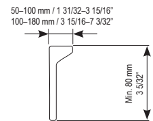
Small clamp for bulb profiles 50-180 mm (option) DCS-0824-0037-02-0
