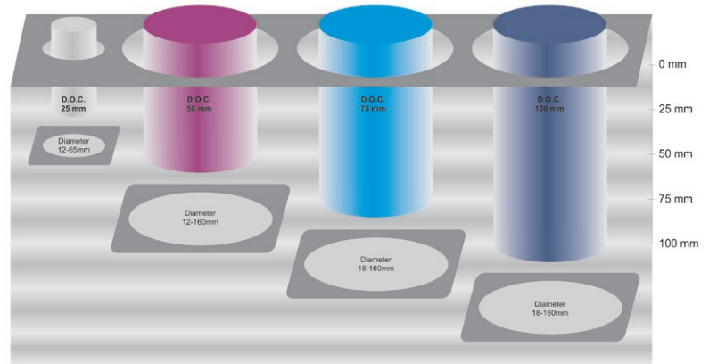
TCT-Kernbohrer
