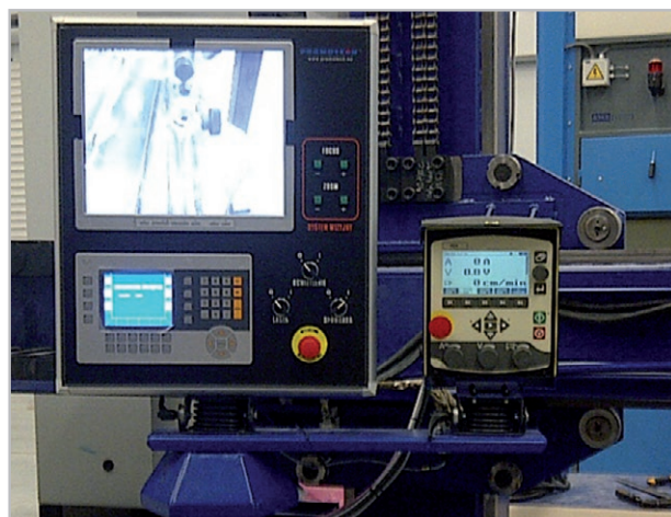
Sample view of CB operating panel and integrated SAW ACDC welding equipment from (Lincoln Electric and ESAB)
