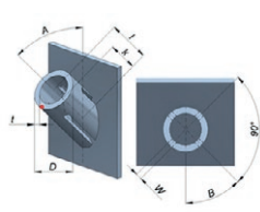
Pipe-plane with holes for fins
