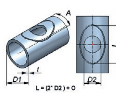
Reinforcement pad
