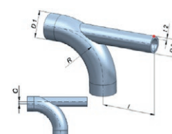
Pipe - elbow
