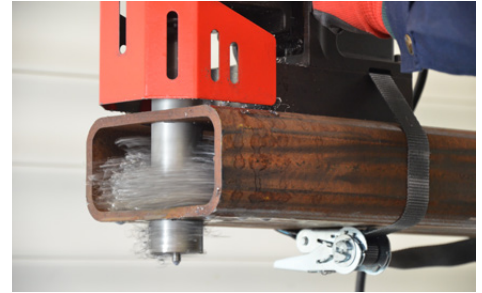
Starting point of milling up to 50 mm (2") below a level of a drill base
