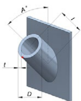
Assemblage tube - plaque
