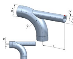
Assemblage tube - coude
